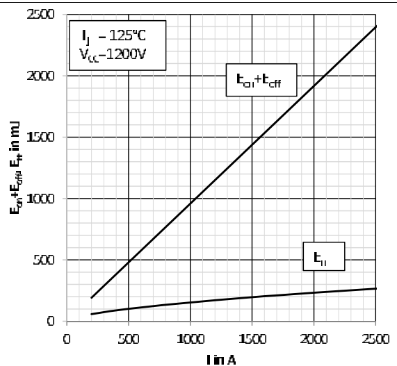
Fig. 4: Typical energy losses E = f(I_C, V_{CE})
