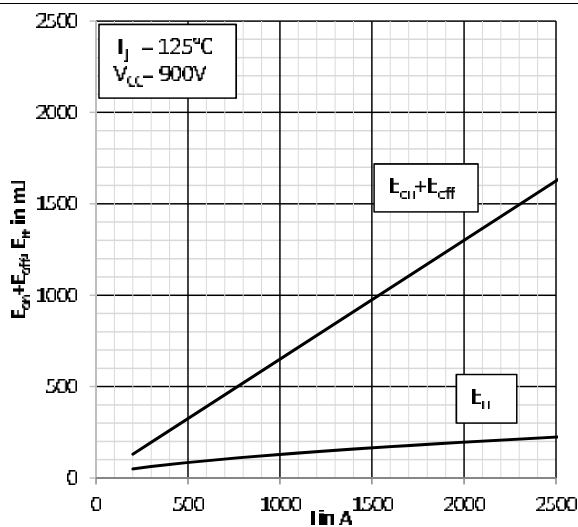
Fig. 3: Typical energy losses E = f(I_C, V_{CE})
